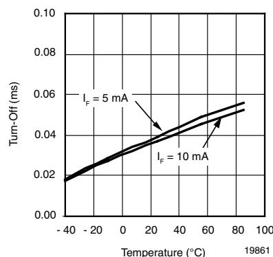
Figure 7. Typical Turn-Off vs. Temperature (Load Current = 100 mA)
