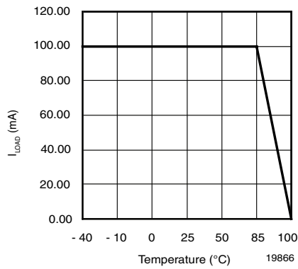
Figure 1. I_{LOAD} vs Temperature
